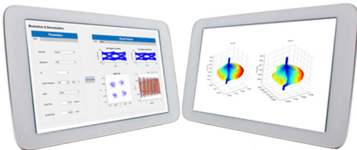
Fig 2.: Example of a digital demodulation as well as an emission measurement of a EUT in the range above 4 GHz
