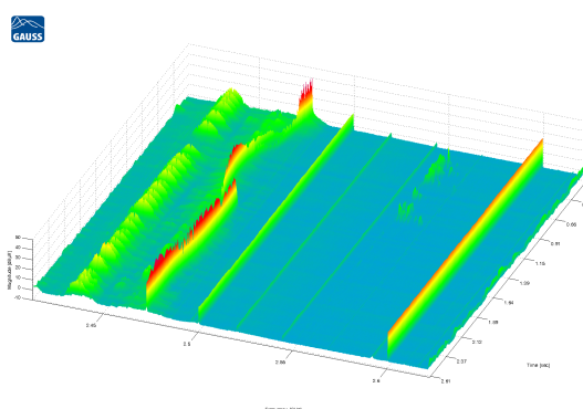
Fig 2.: Measurement of several communication signals and signal of a microwave oven with 100-fold HyperOverlapping
